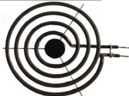
▲ Universal 3-Turn Plug-In Range Elements 69750 - 6" Wide- 1250 Watt 69751 - 8" Wide- 2100 Watt
